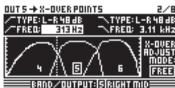
Abb. 3.2: Out \Rightarrow X-Over Points
